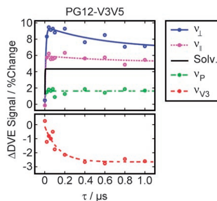
Figure 4. Transient DVE signal of PG12-V3V5 at four frequency channels. Each data point is the average of over the following frequency ranges: 1558–1567 \text{cm}^{-1} (red), 1598–1607 \text{cm}^{-1} (green), 1639–1648 \text{cm}^{-1} (violet), 1668–1678 \text{cm}^{-1} (blue). The fitted transient absorbance of the solvent is scaled by 150 and plotted in black. Open circles correspond to measured data, and the lines are single exponential fits to the data. The \tau_1 rise time of the fits to the \nu_{\perp} , \nu_{\parallel} , and \nu_{\text{P}} data is less than 10 ns, and the fitted \tau_1 decay time of the \nu_{\text{V3}} peak is 135 \pm 50 \text{ ns} . The \nu_{\perp} and \nu_{\parallel} signals each have subsequent decay times of 610 and 680 ns, respectively.
